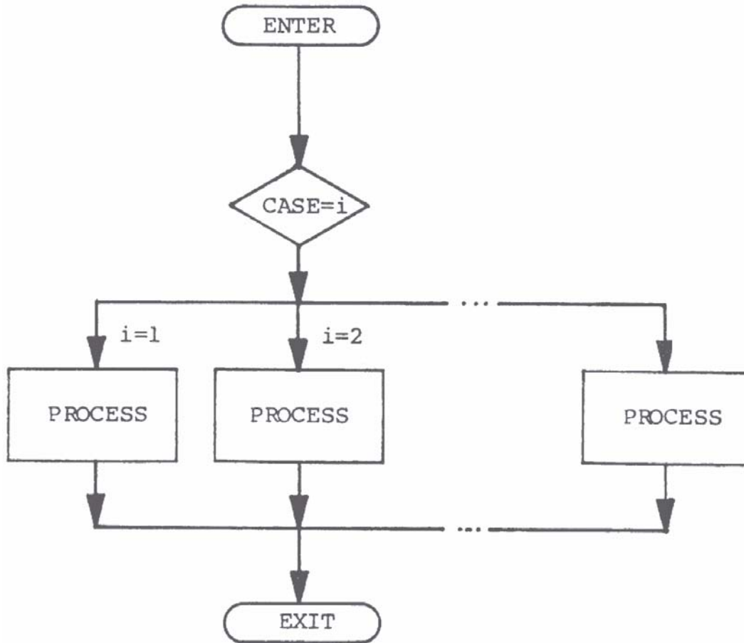
Figure 5 CASE
