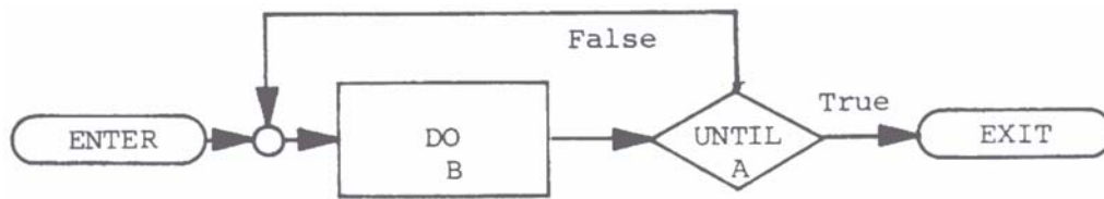
Figure 4 DO-UNTIL
